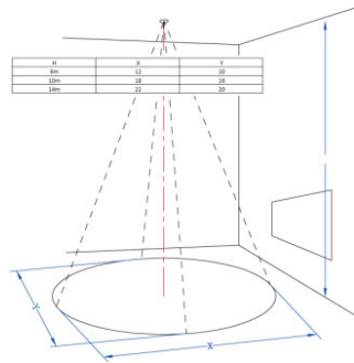
Detection area vs height QBM 220 240 LS PD HB CI
